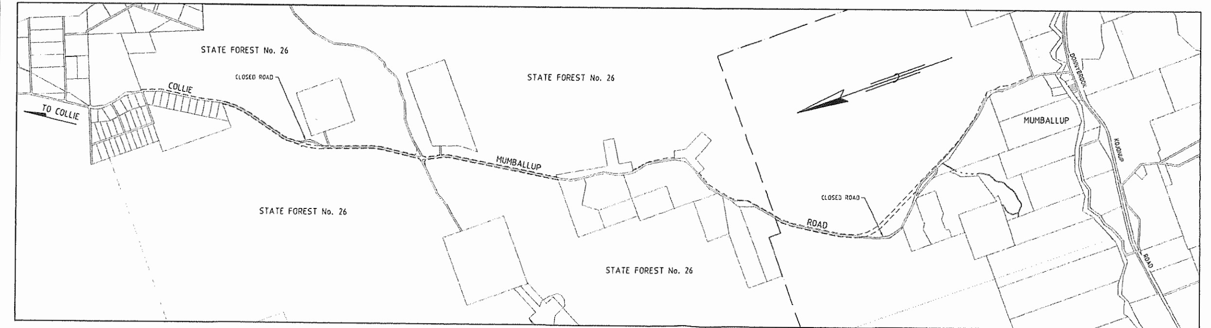
LOCALITY PLAN SCALE 1:25000
